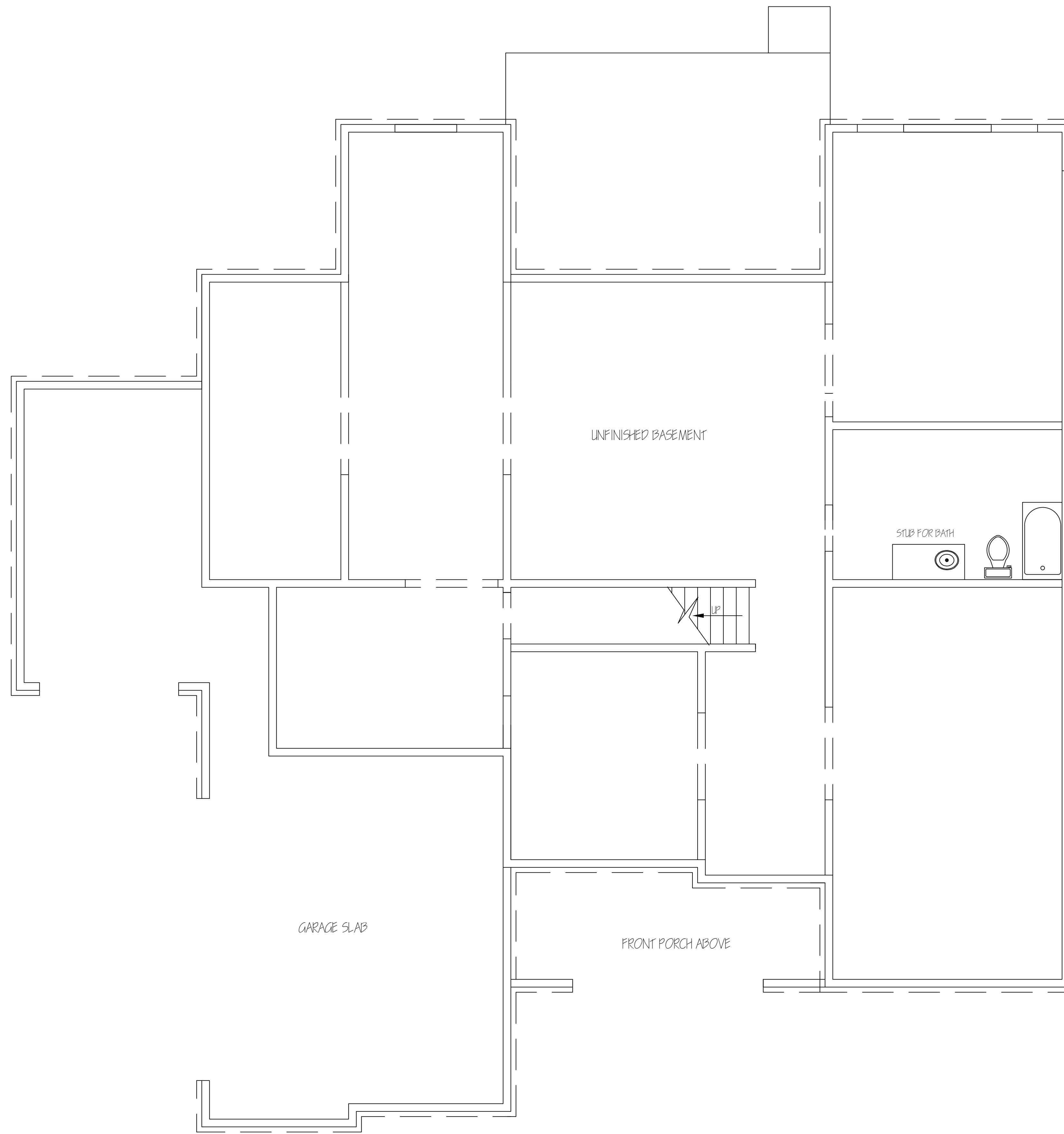
1 BASEMENT FOUNDATION PLAN
