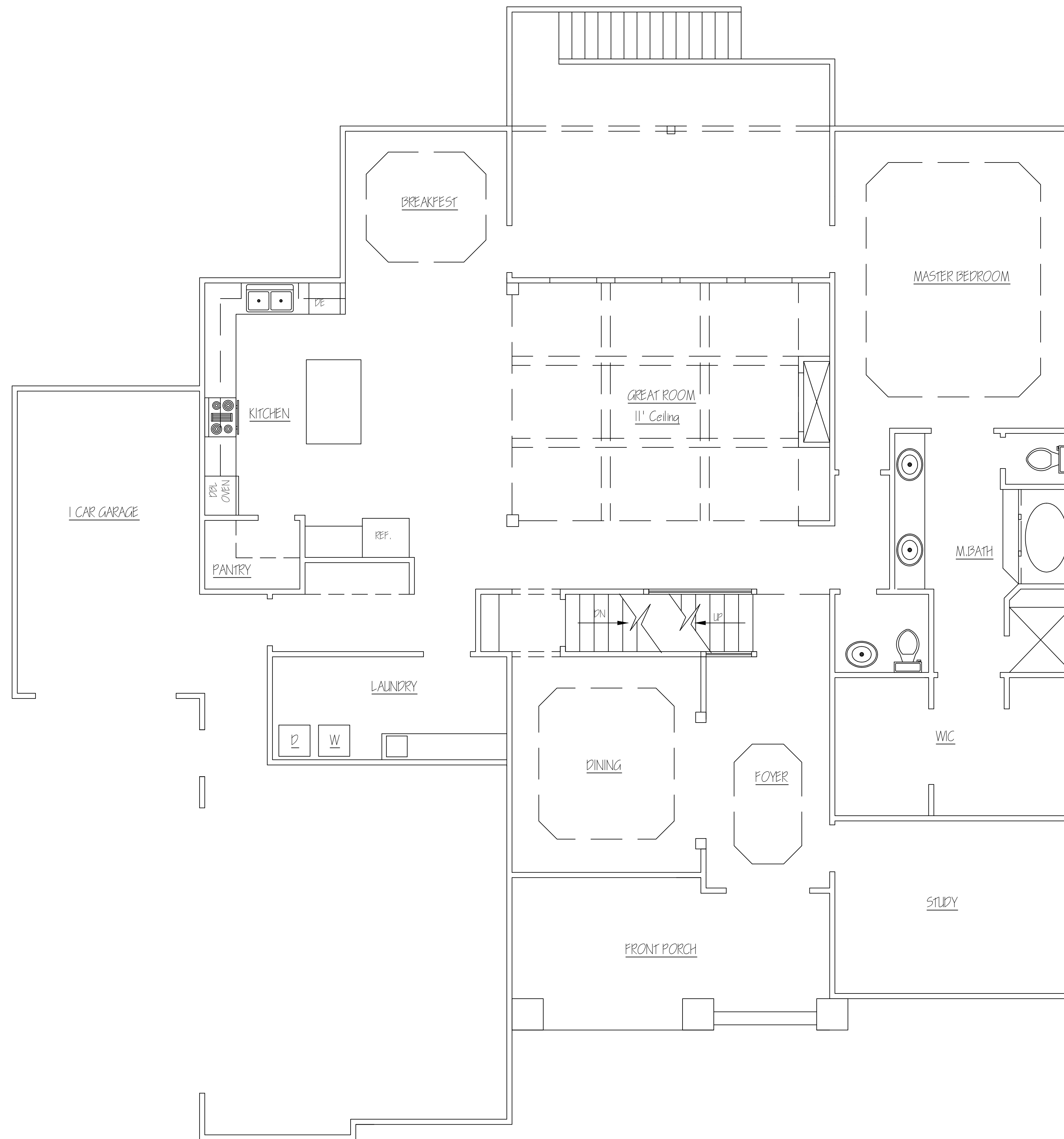
1 MAIN LEVEL FLOOR PLAN
